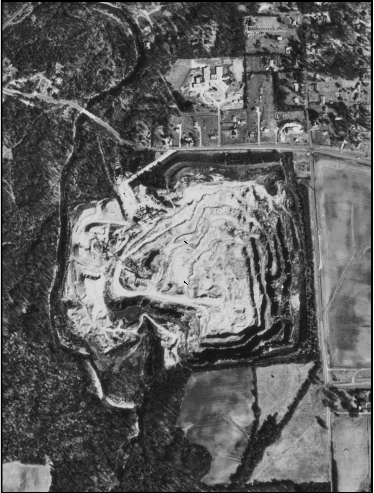
FIGURE 4 ELK MILLS QUARRY AERIAL PHOTOGRAPH - EXISTING CONDITIONS
