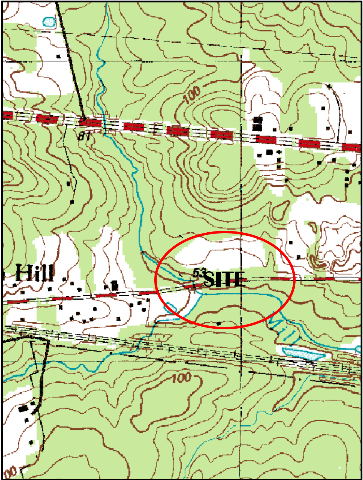
FIGURE 29 MILL CREEK (EAST) POTENTIAL RESERVOIR EXISTING TOPOGRAPHY
