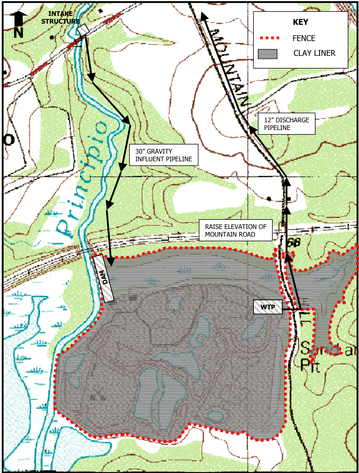
FIGURE 20 PRINCIPIO CREEK POTENTIAL OFF-LINE RESERVOIR LAYOUT
