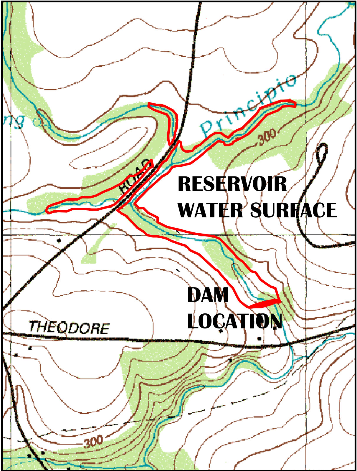
FIGURE 14 PRINCIPIO CREEK POTENTIAL ON-LINE RESERVOIR LAYOUT
