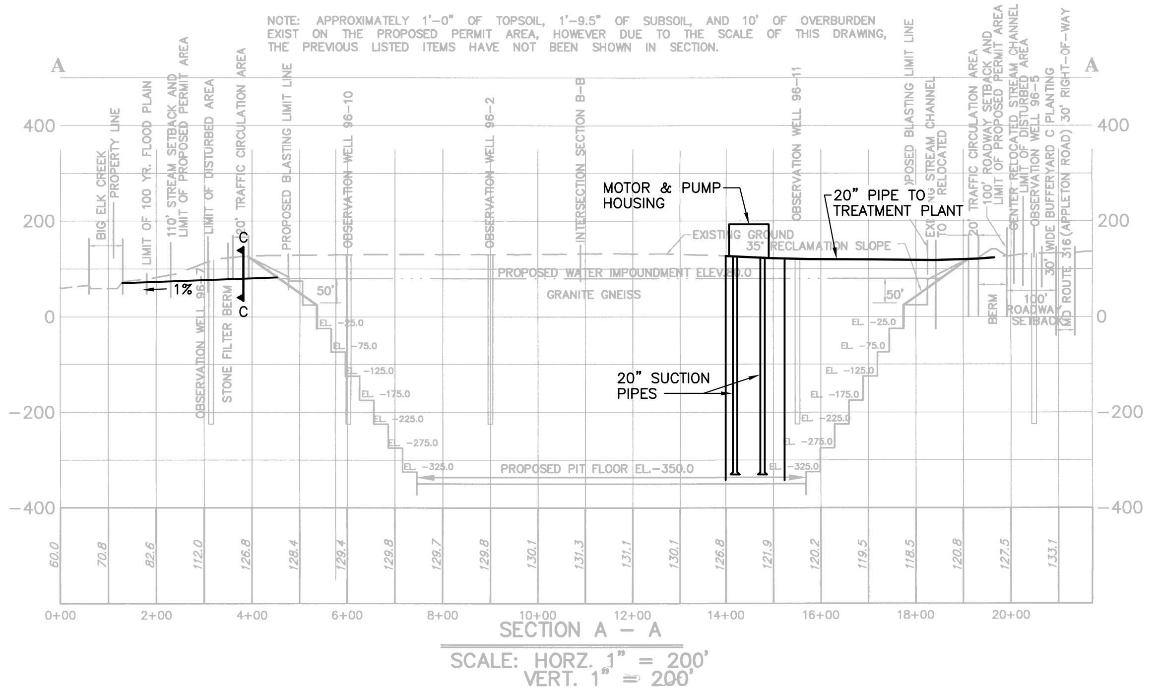
FIGURE 10 ELK MILLS QUARRY POTENTIAL RESERVOIR & TREATMENT PLANT CROSS SECTION
